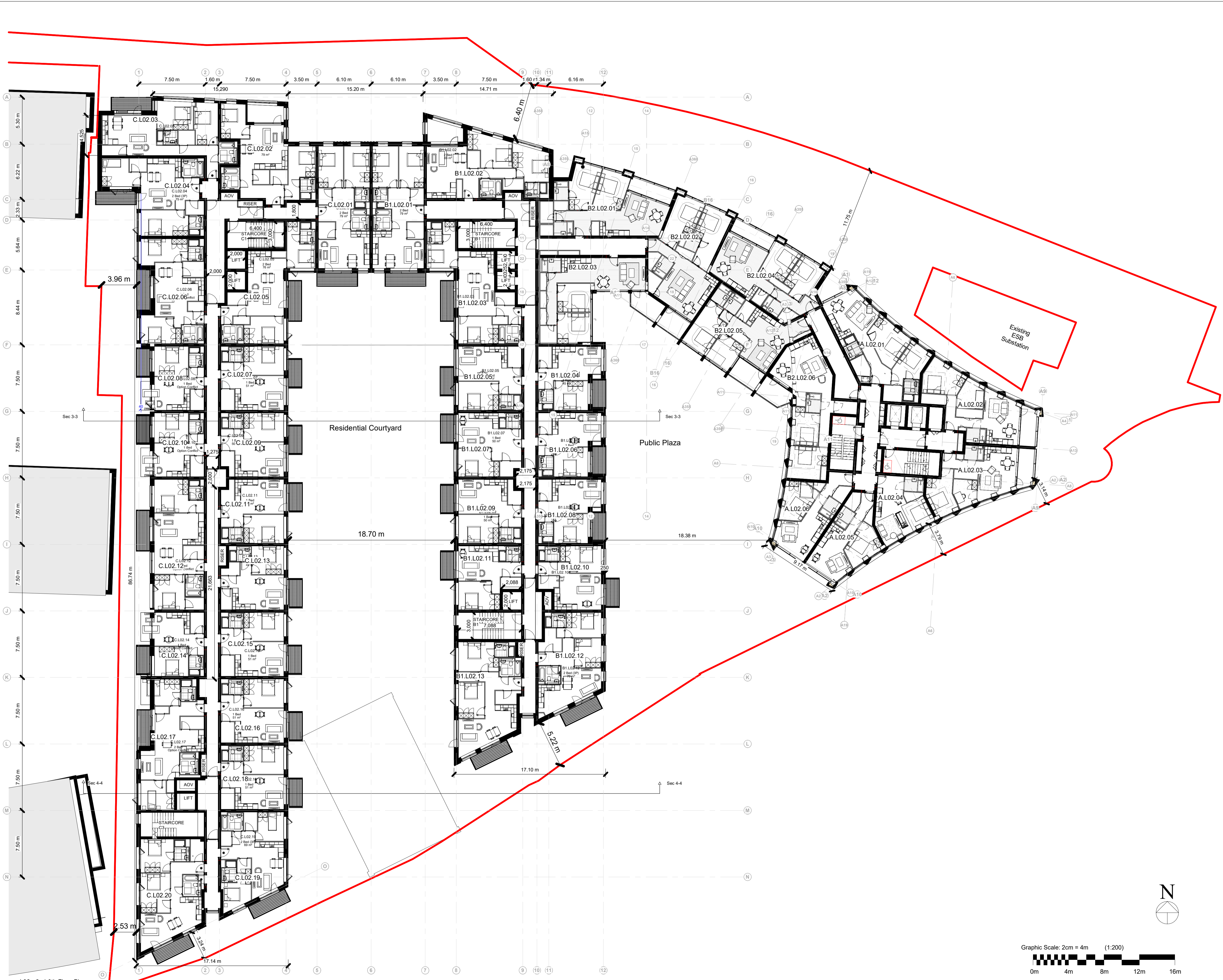
L02 - 2nd-6th Floor Plan 1 : 200
