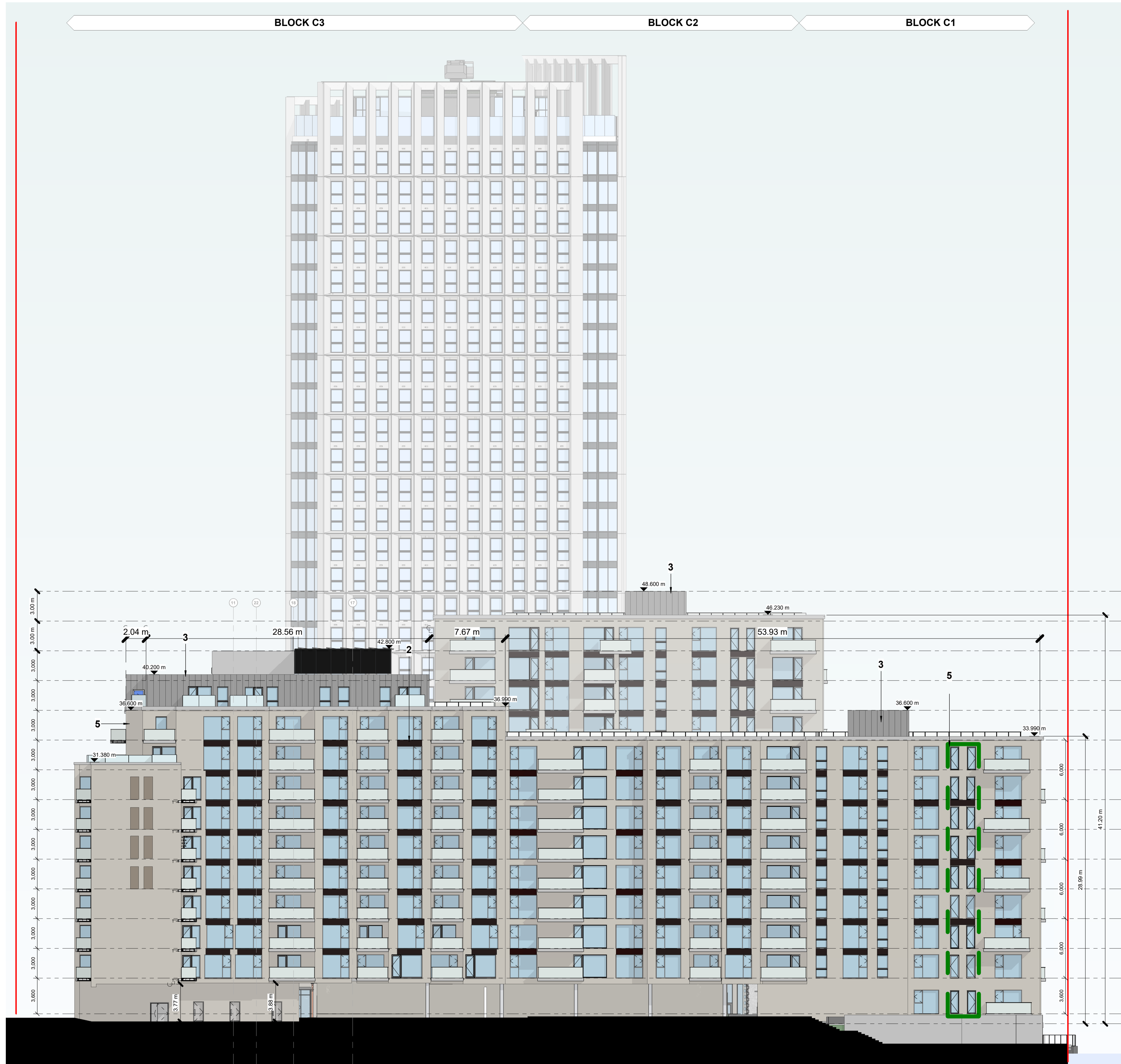
Proposed West Elevation 1 : 200
