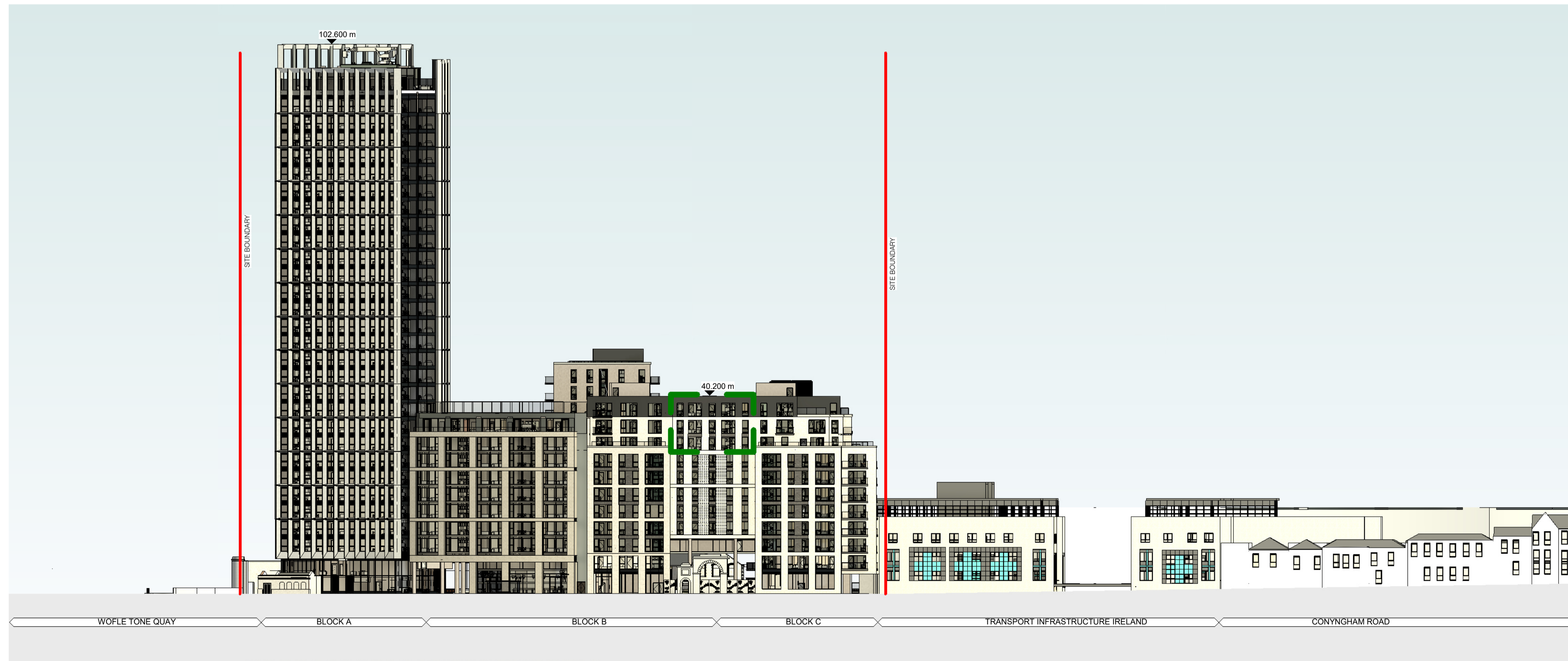
North Contextual Elevation 1 : 500
