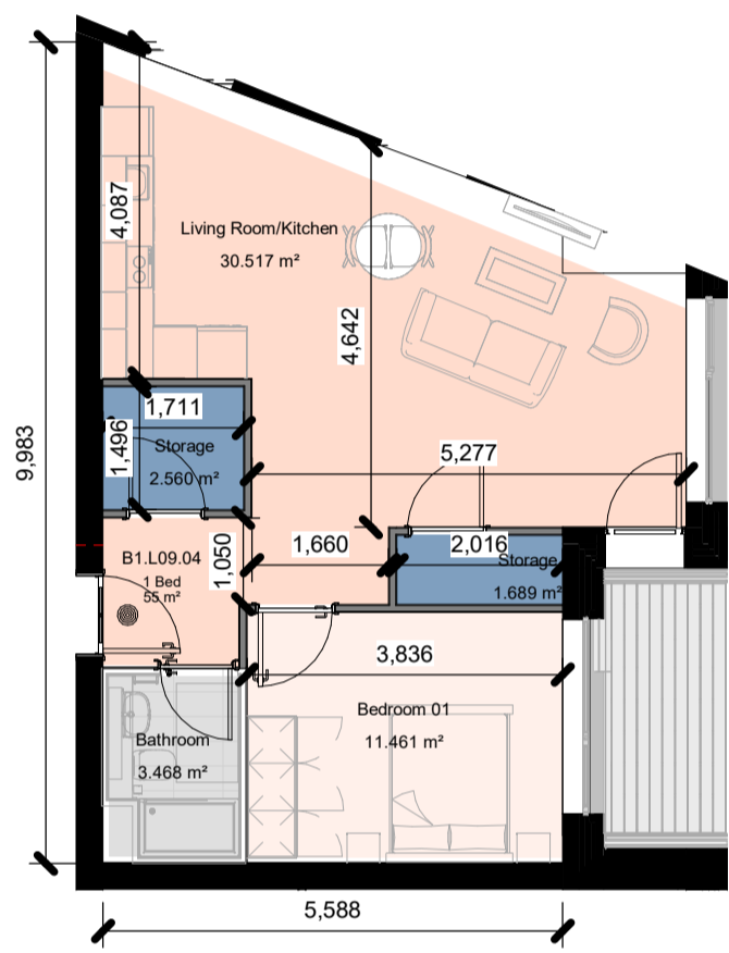
Apt Type 1Bed (W)-9th-10th-11th Floor 1 : 100
