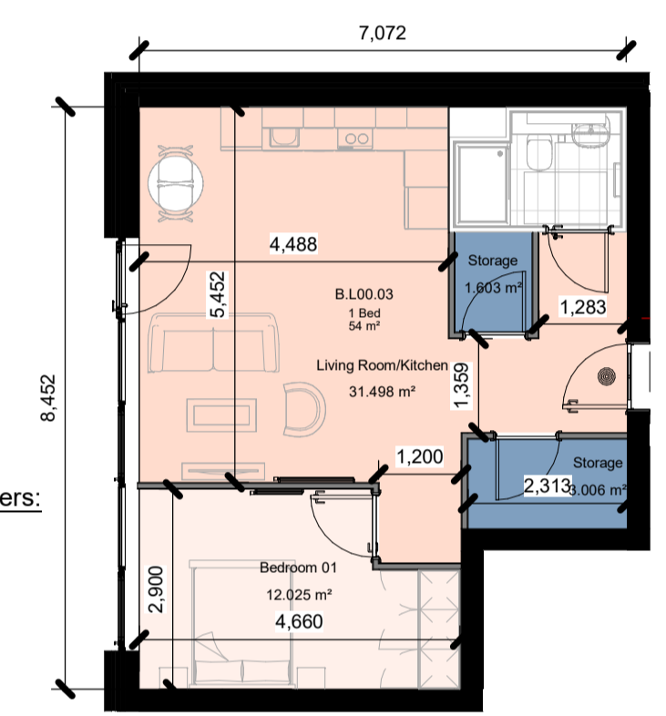
Apt Type 1Bed (Y)-Ground Floor 1 : 100
