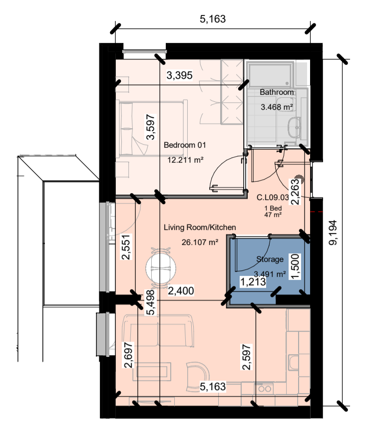
Apt Type 1Bed (T)-9th Floor 1 : 100
